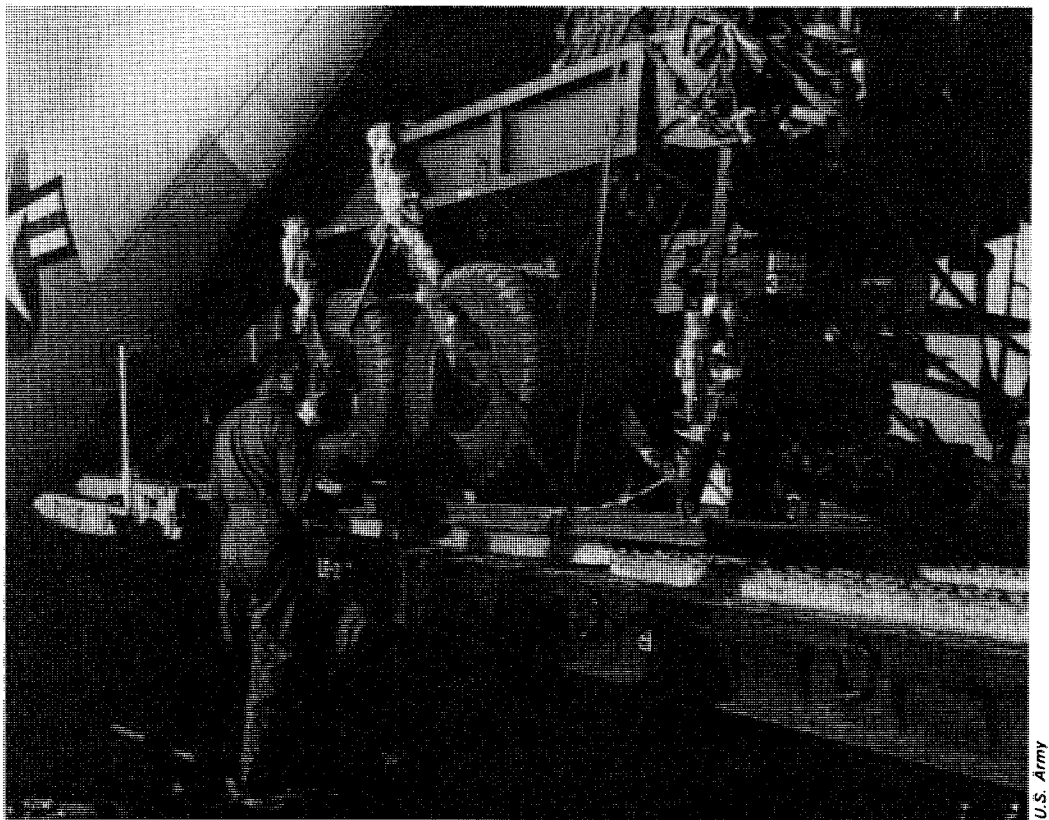
A 2½-ton truck being rigged and loaded for airdrop aboard a C-130 transport
